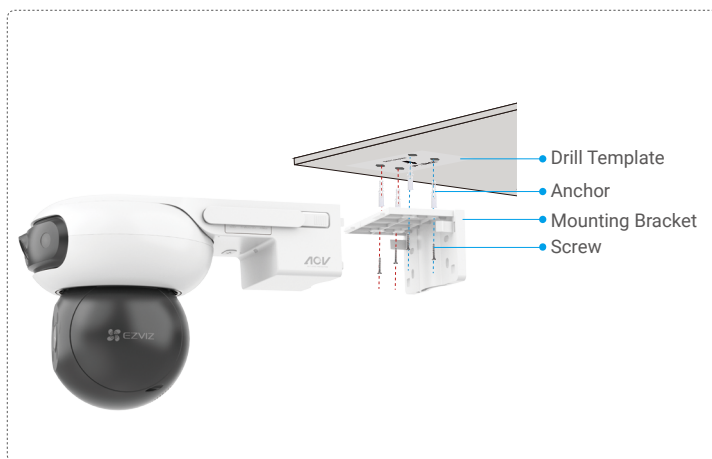
Fig. 1 Ceiling Mount
